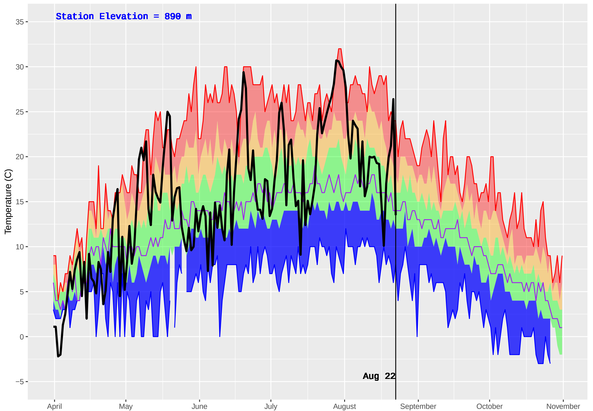
ISKUT (112) : Historical (1979–2016) and Current (2018) Daily Temperature
