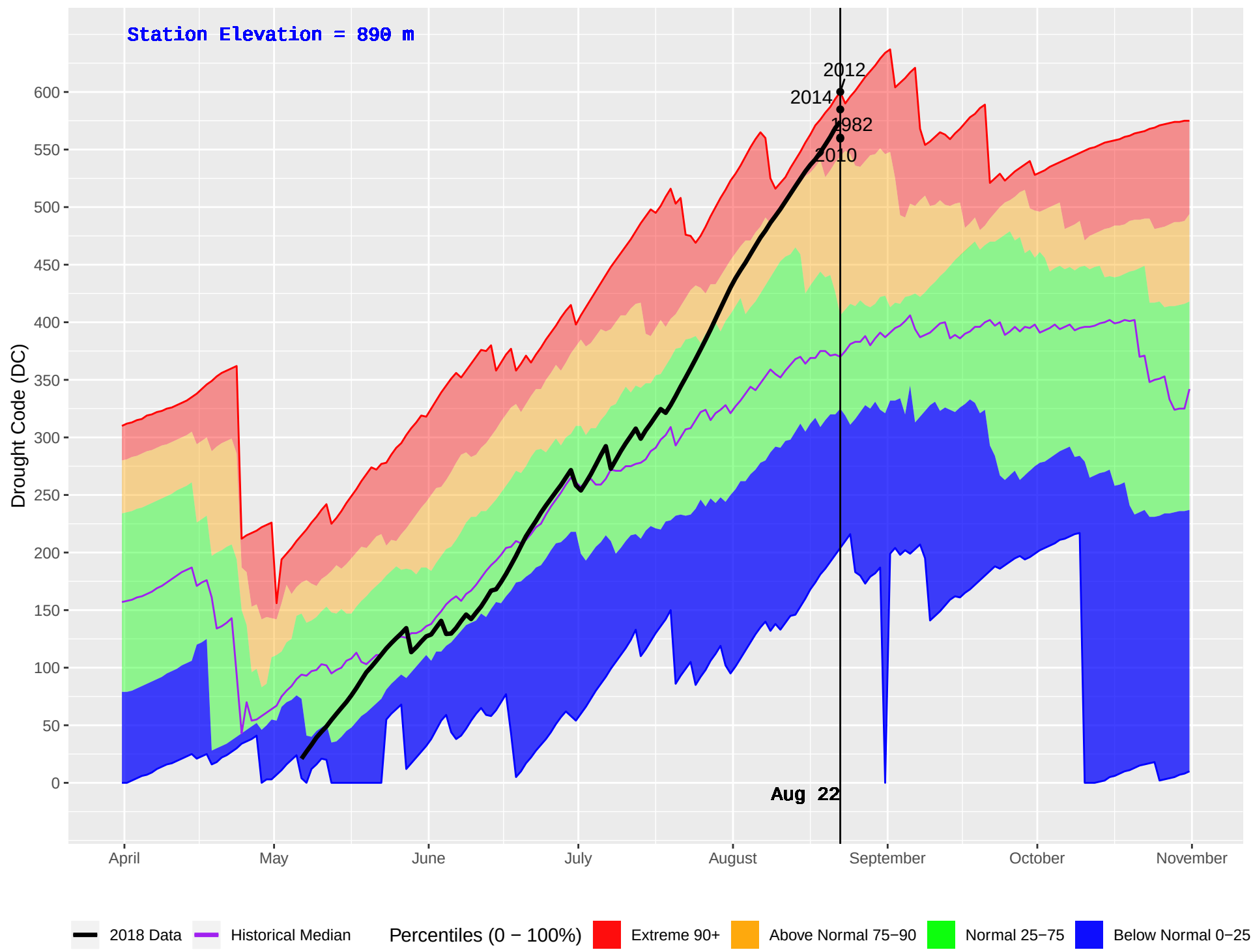
ISKUT (112) : Historical (1979–2016) and Current (2018) Daily Drought Code (DC)
