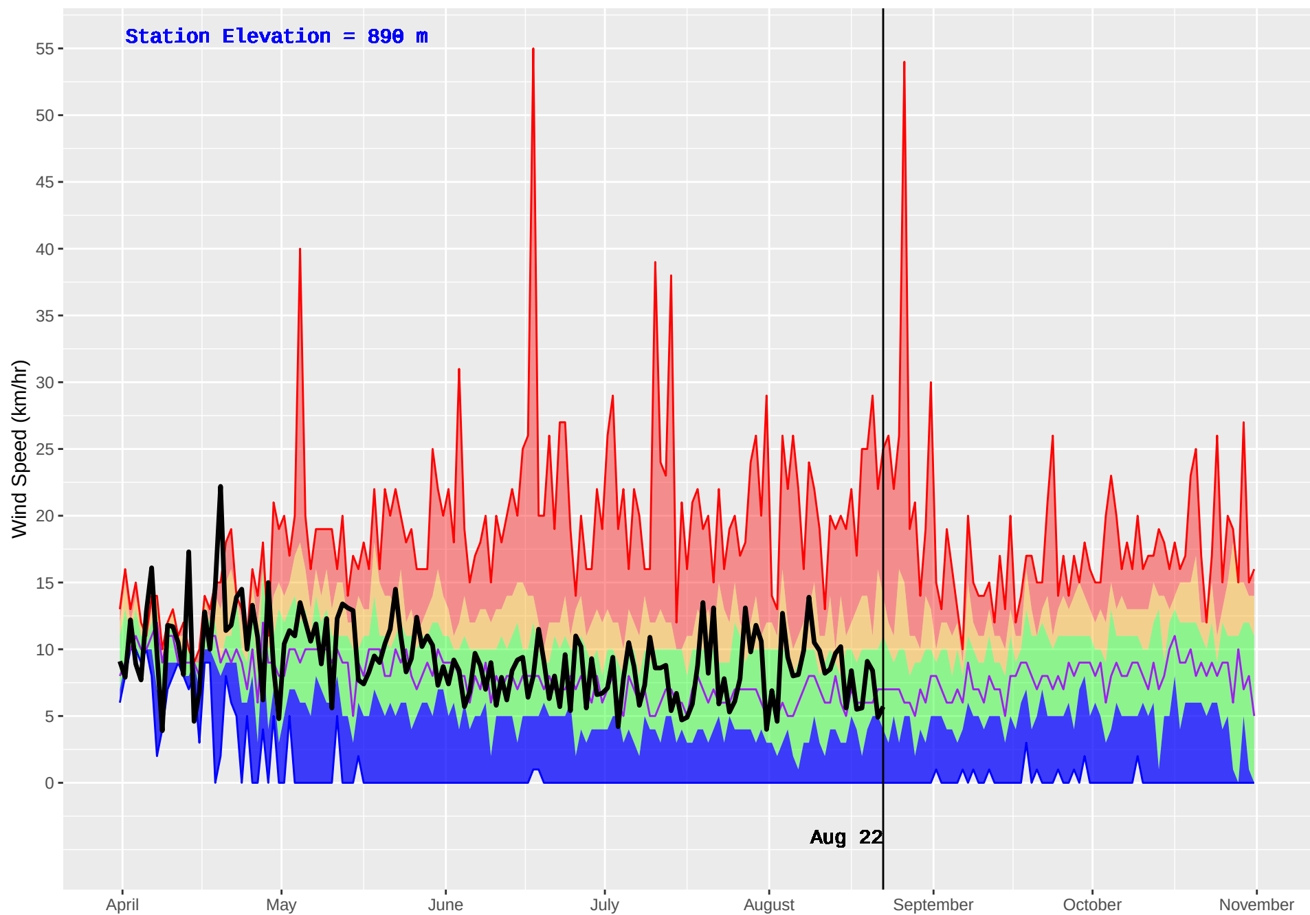
ISKUT (112) : Historical (1979–2016) and Current (2018) Daily Wind Speed
